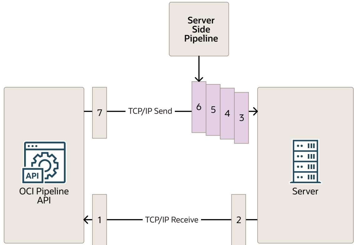
Figure 22-4 OCI Pipeline Block Diagram
