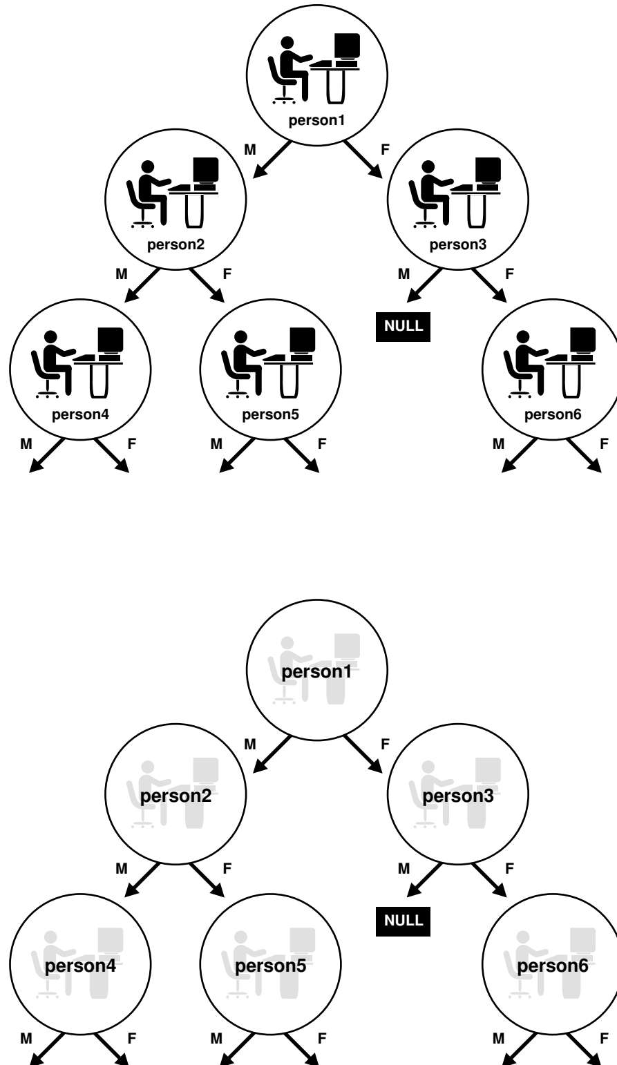
Figure 21-2 Object Graph of person_t Instances
