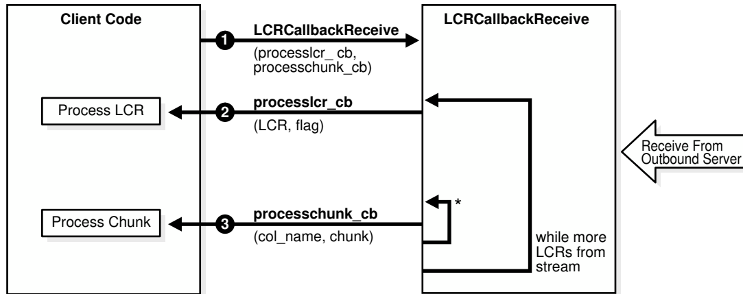
Figure 36-2 Execution Flow of the OCIXStreamOutLCRCallbackReceive() Function
