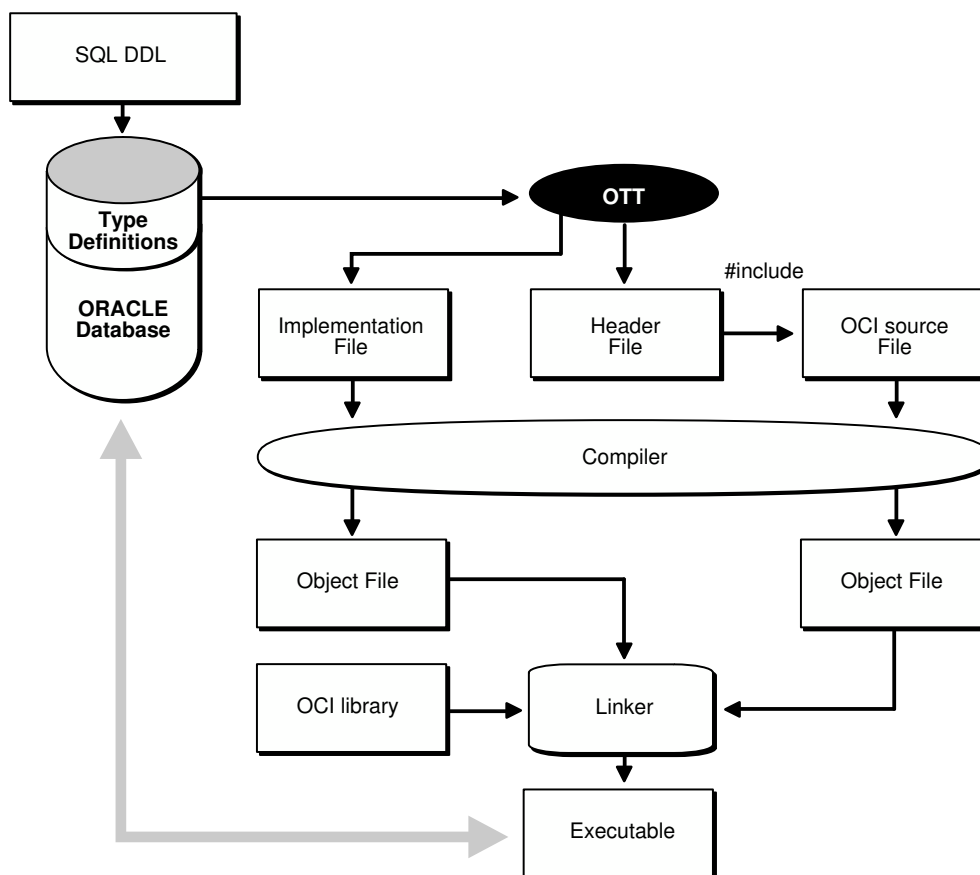
Figure 25-1 Using OTT with OCI
