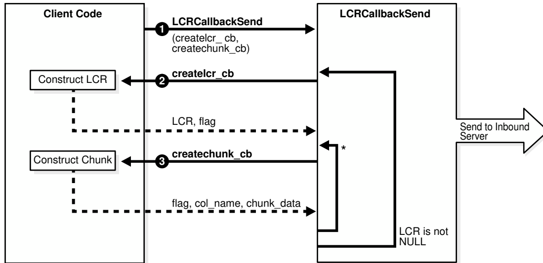
Figure 36-1 Execution Flow of the OCIXStreamInLCRCallbackSend() Function
