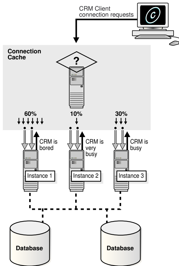
Figure 6-1 Run-time Connection Load Balancing
