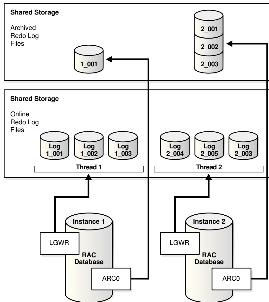
Figure 4-7 Illustration of Redo Threads for an Oracle RAC Database
