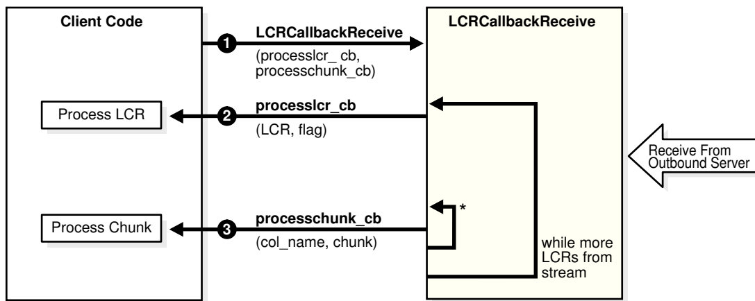
Figure 26-2 Execution Flow of the OCIXStreamOutLCRCallbackReceive() Function
