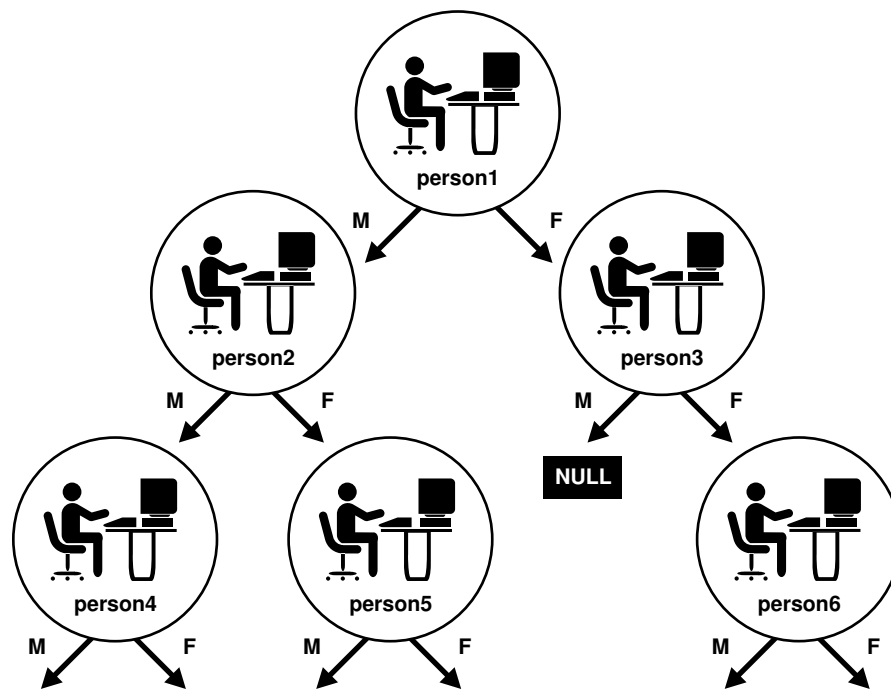
Figure 14-2 Object Graph of person_t Instances
