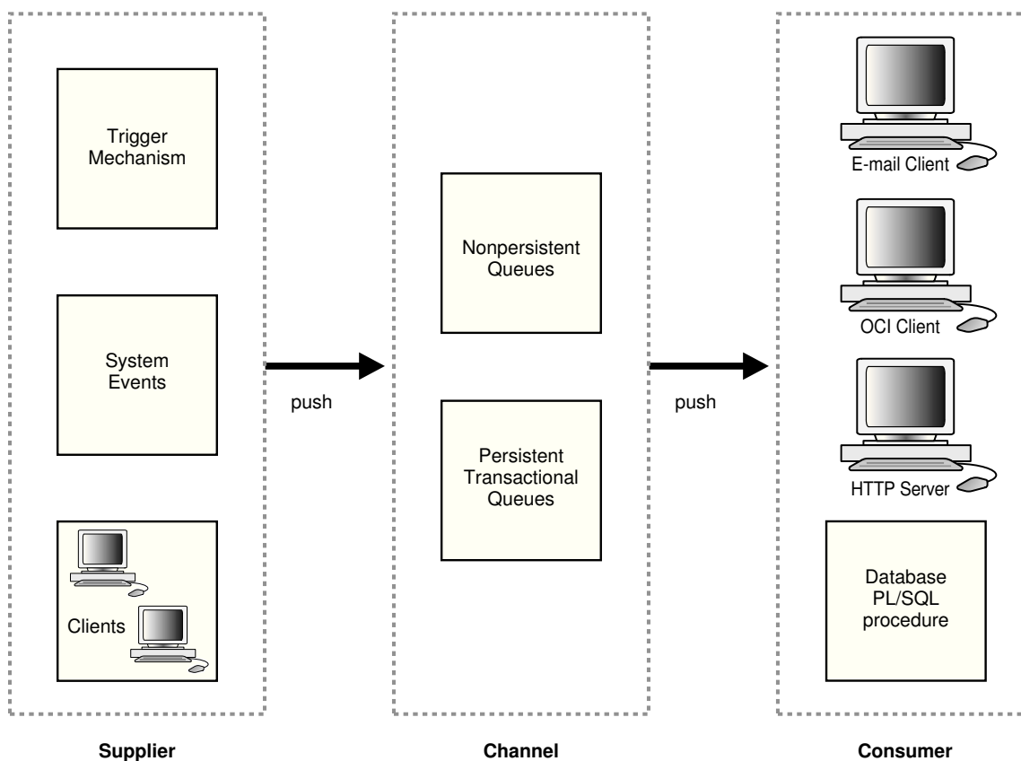
Figure 9-2 Publish-Subscribe Model
