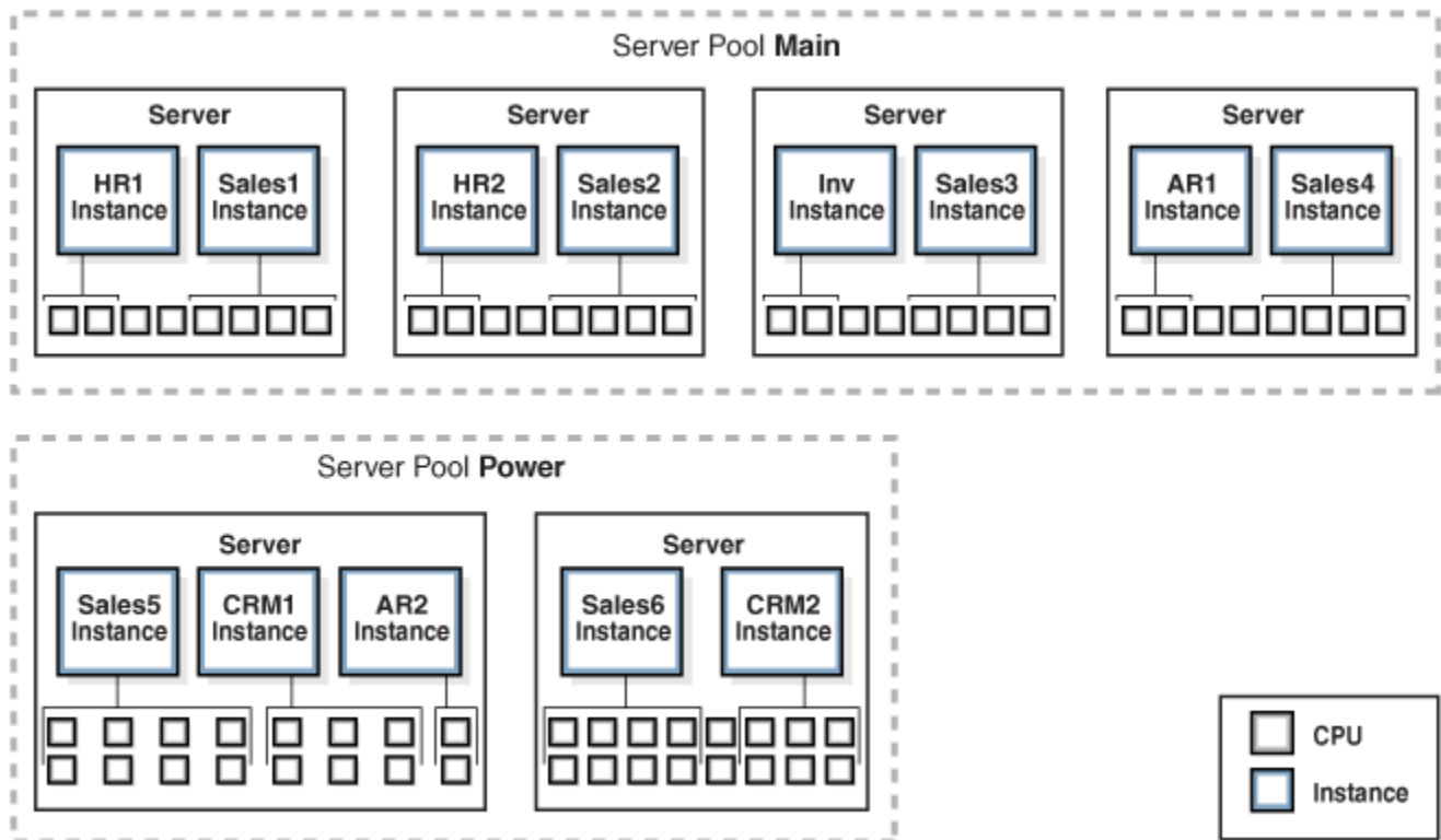
Figure 1-4 Server Pools and CPU Slices
