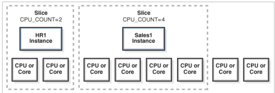
Figure 1-1 Instance Caging and CPU Slices
