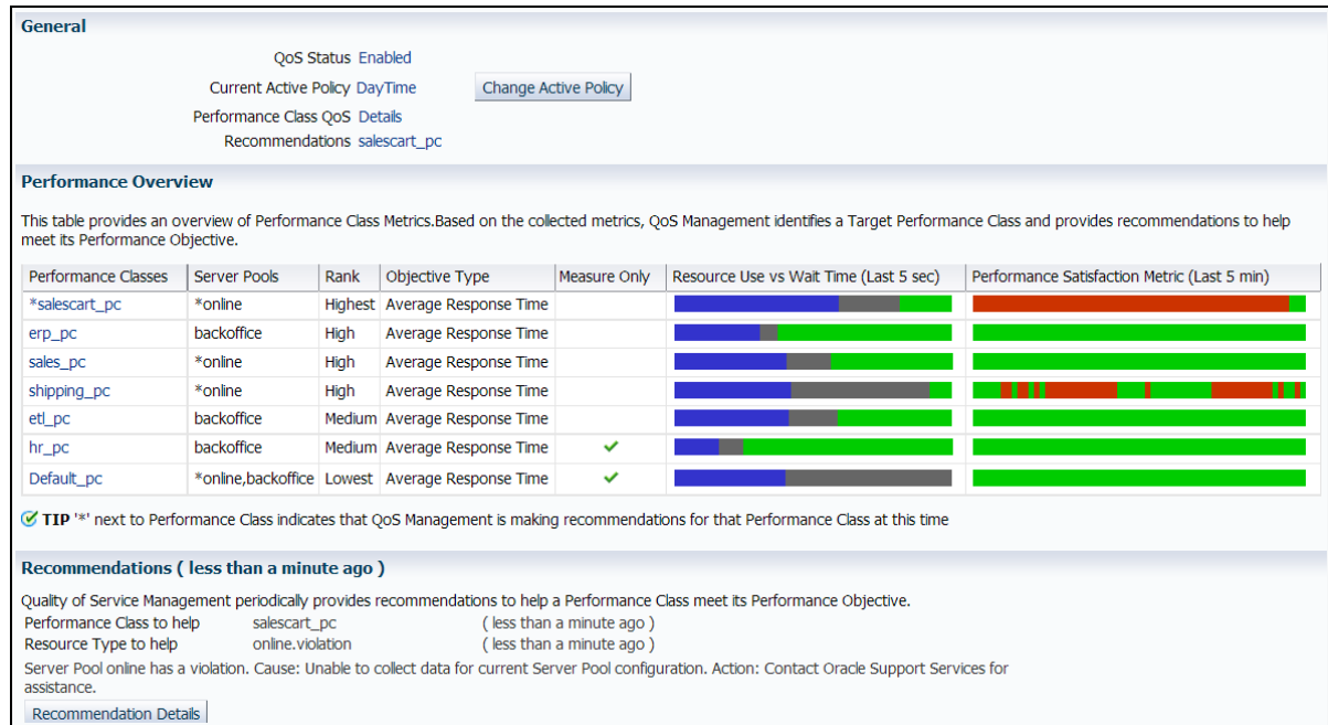
Figure 4-2 Oracle Database Quality of Service Management Dashboard
