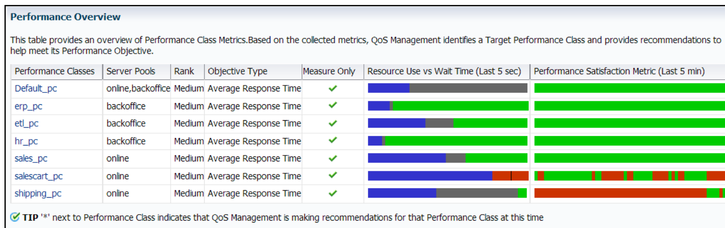
Figure 4-1 Performance Satisfaction Metrics for Measure-Only Performance Classes
