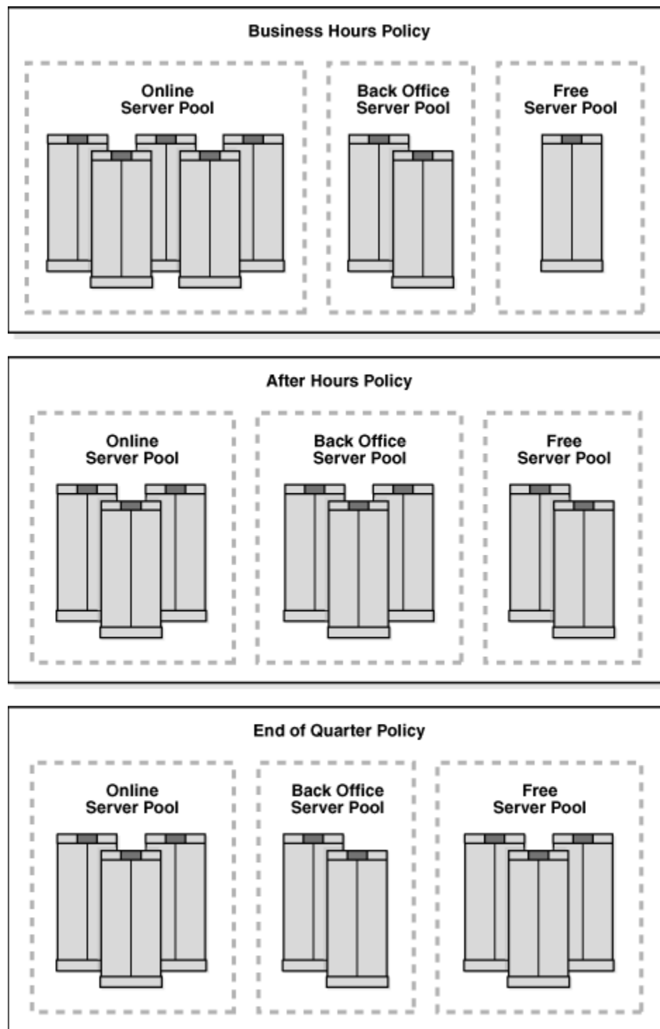
Figure 1-5 Baseline Resource Management by Performance Policy
