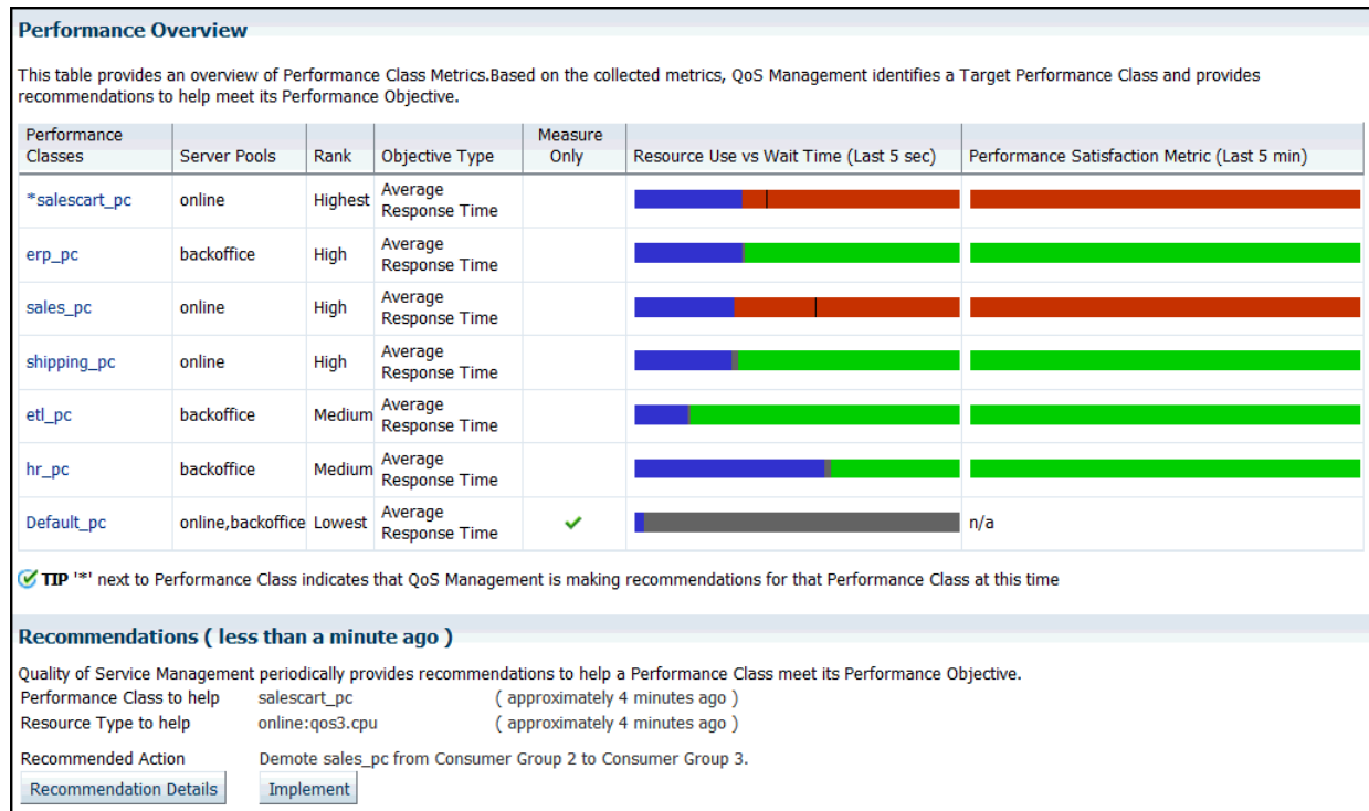
Figure 4-4 Performance Overview Page Showing Performance Classes Not Meeting Their Performance Objectives
