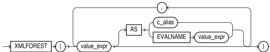
Figure 8-3 XMLFOREST Syntax
