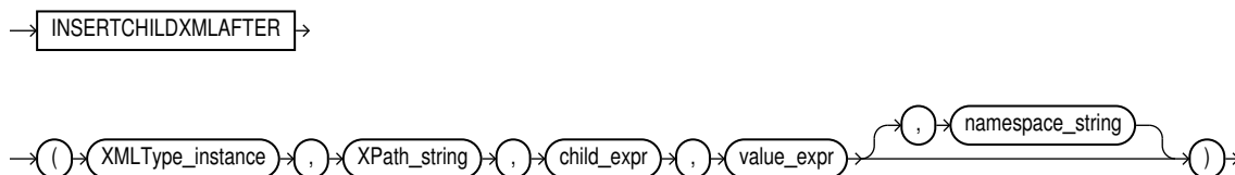
Figure C-4 INSERTCHILDXMLAFTER Syntax
