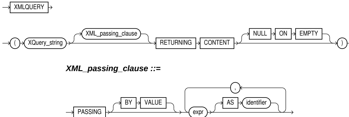
Figure 4-1 XMLQUERY Syntax
