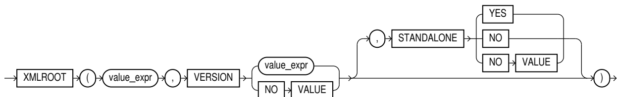
Figure 8-10 XMLRoot Syntax
