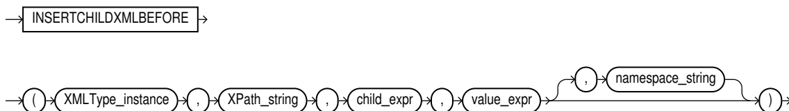
Figure C-3 INSERTCHILDXMLBEFORE Syntax
