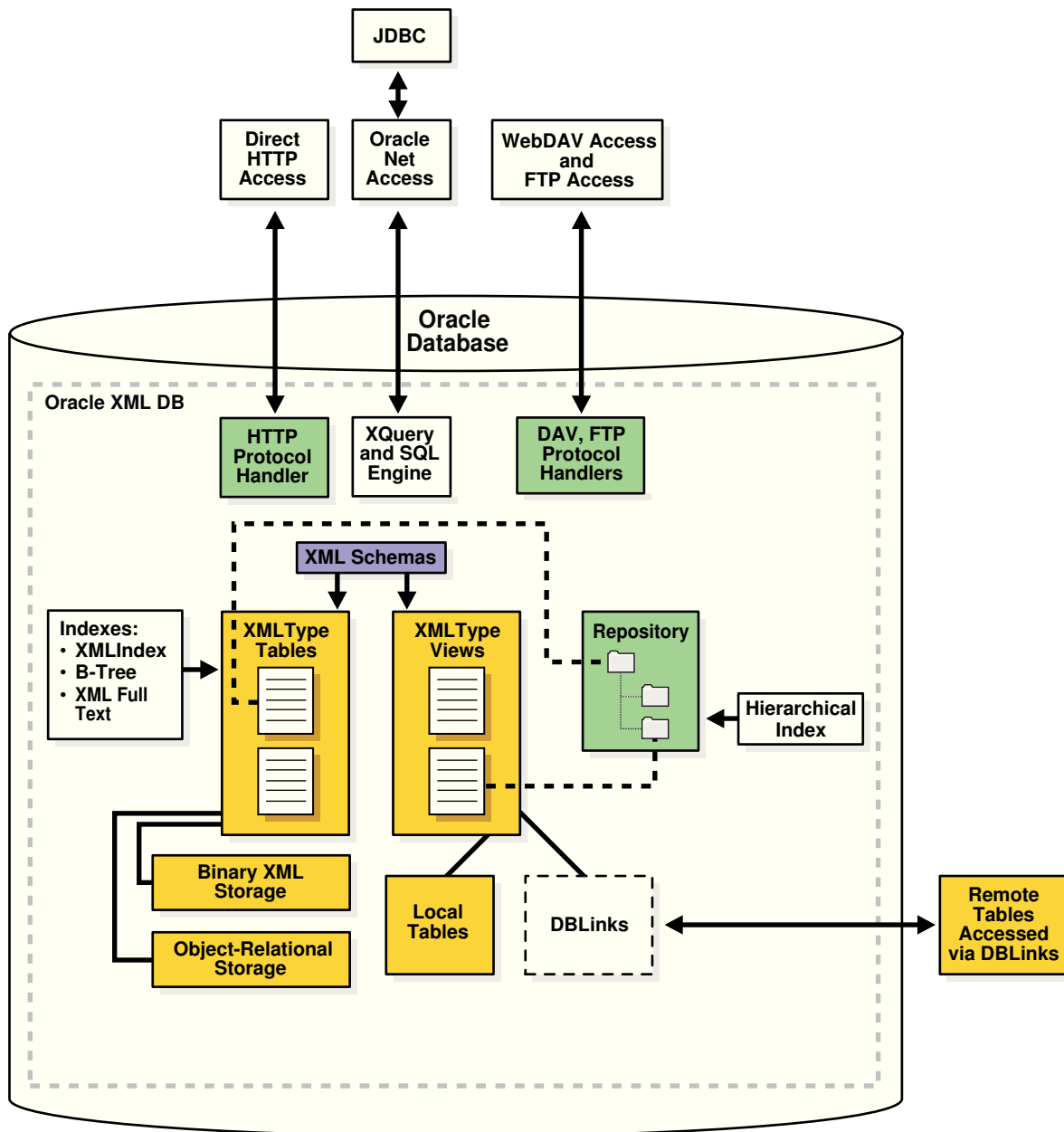
Figure 1-3 XMLType Storage
