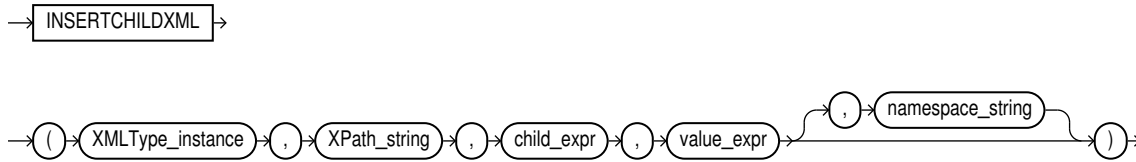
Figure C-2 INSERTCHILDXML Syntax
