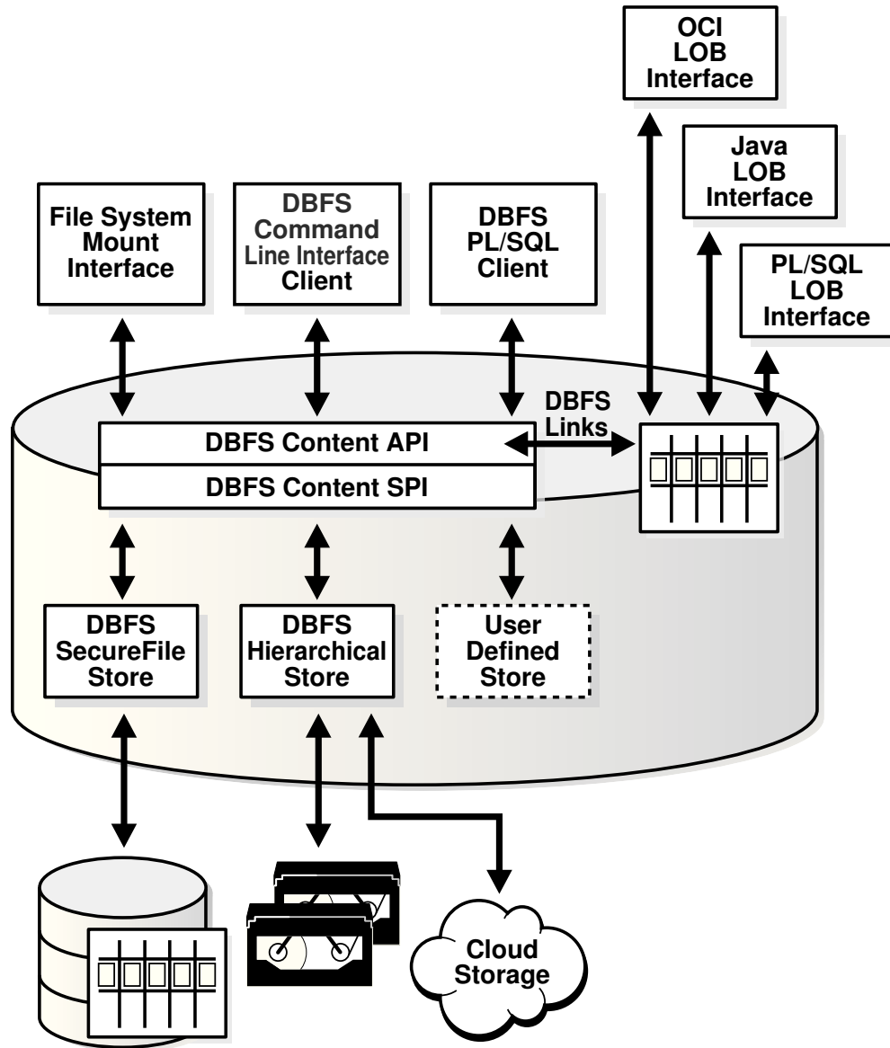
Figure 9-1 Database File System (DBFS)
