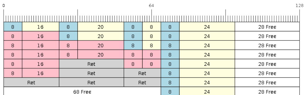
Fig. 41: Retrieving/Returning items in No-Split and Allow-Split ring buffers
