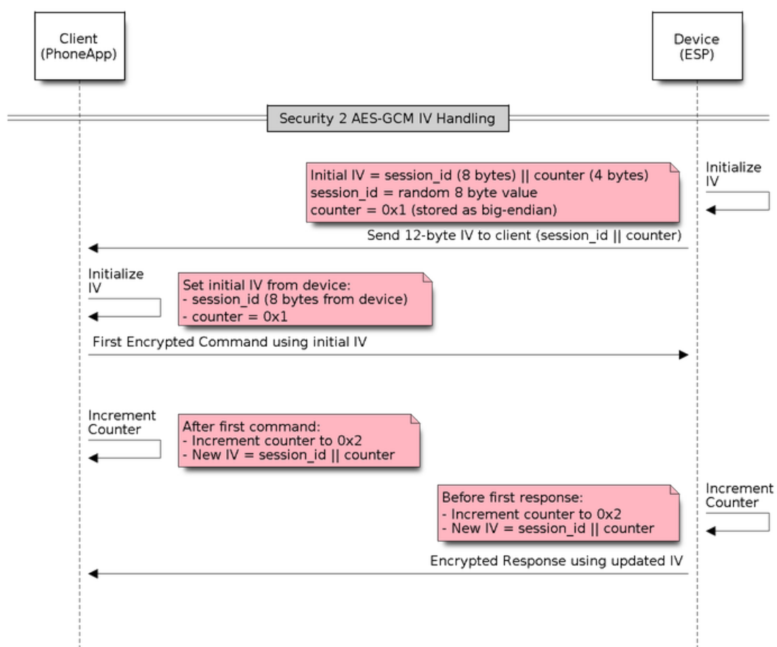
Fig. 34: Security 2 AES-GCM IV Handling
