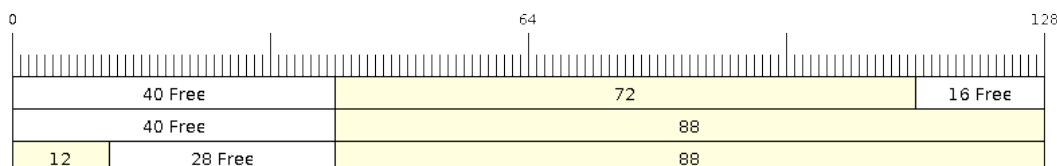
Fig. 40: Wrap around in byte buffers
