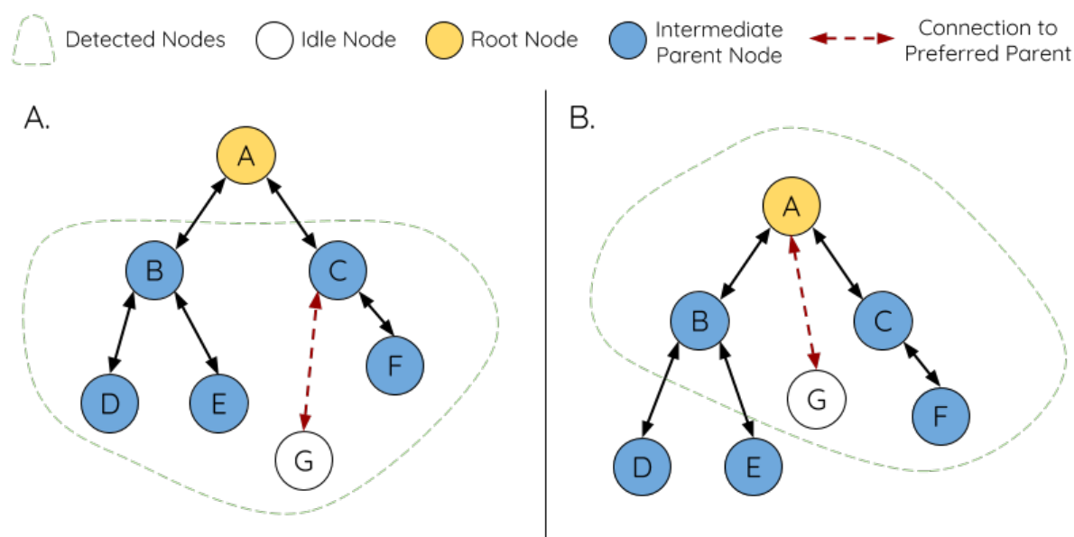
Fig. 47: Preferred Parent Node Selection
