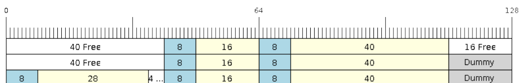
Fig. 38: Wrap around in No-Split buffers
