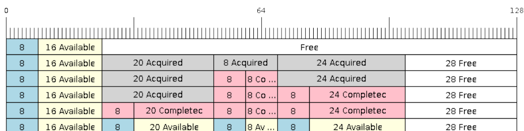
Fig. 37: SendAcquire/SendComplete items in No-Split ring buffers
