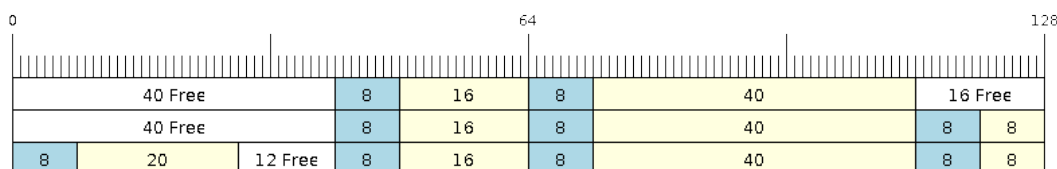
Fig. 39: Wrap around in Allow-Split buffers
