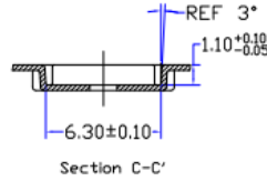
Section C-C'
